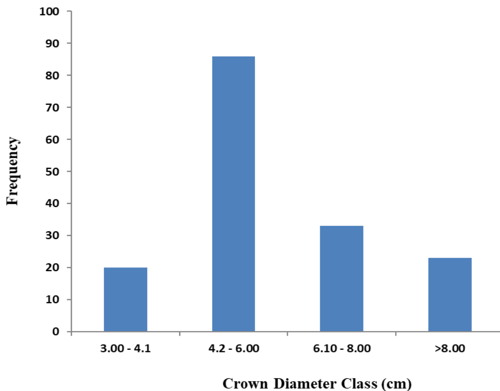
Figure 3: Crown Diameter Class Distribution of Madrid Tree Species ( P. erinaceus ) in the Study Area
