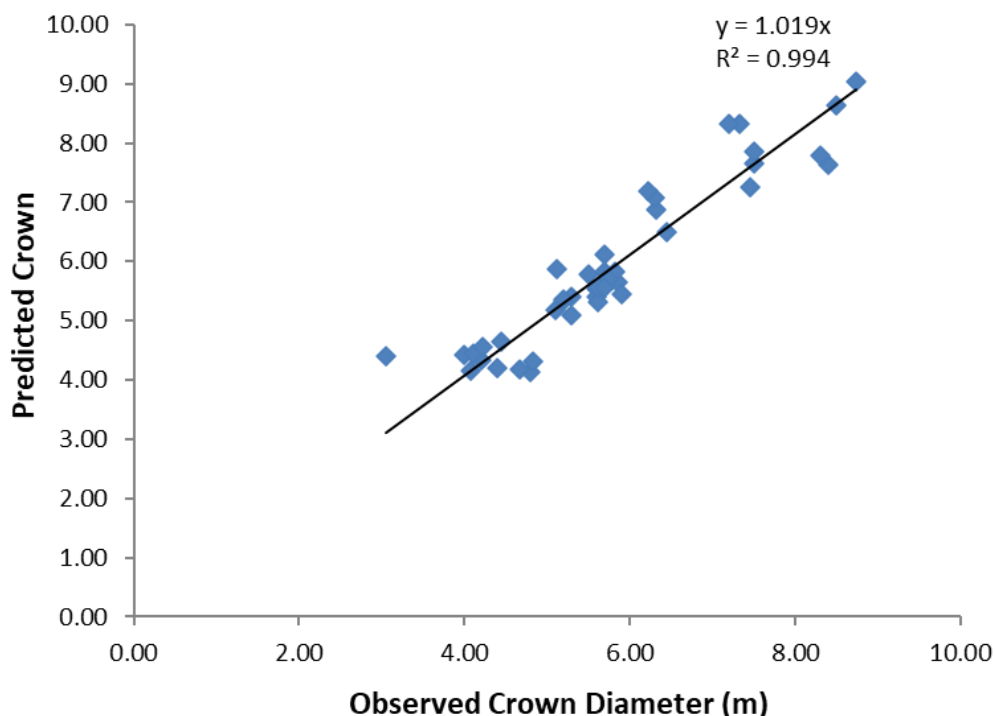
Figure 4: Correlation between Observed and Predicted Crown Diameter of Madrid Tree Species ( P. erinaceus ) in Okpoga, Nigeria
