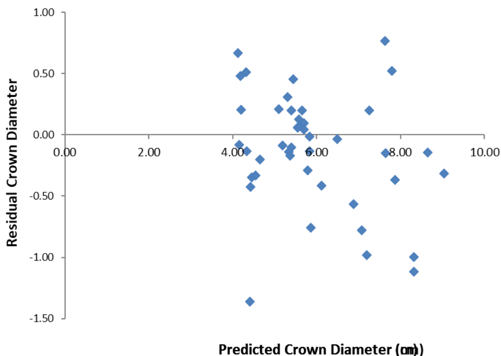
Figure 5: Residual Plot of Madrid Tree Species ( P. erinaceus ) in Okpoga, Nigeria
